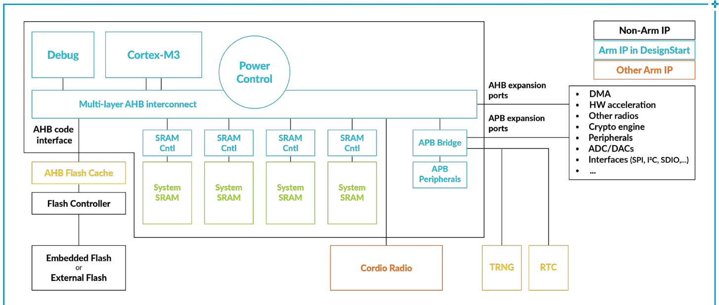
Figure 4: SSE-050 subsystem block diagram
