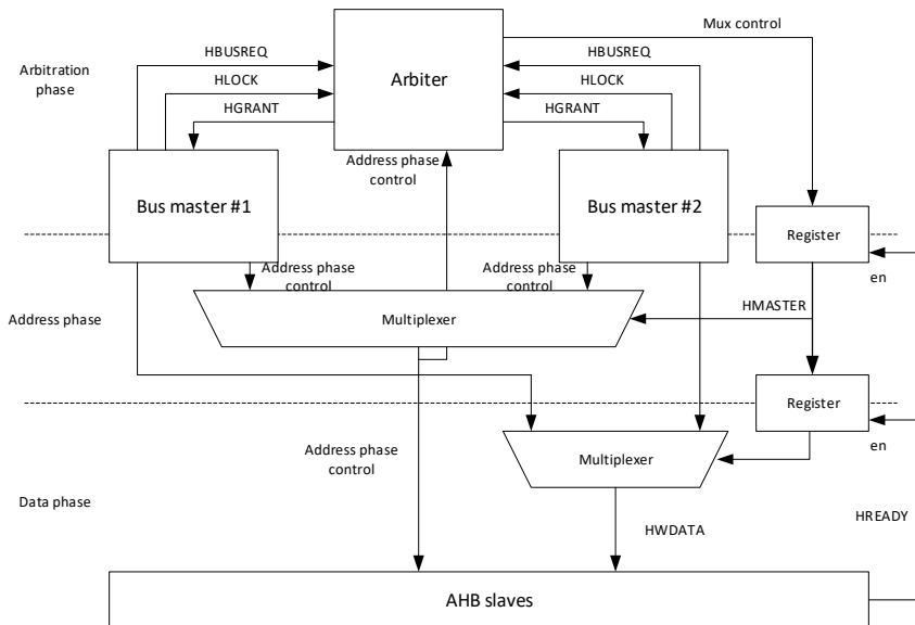
Figure 3.14: Example of arbiter with two bus masters.
