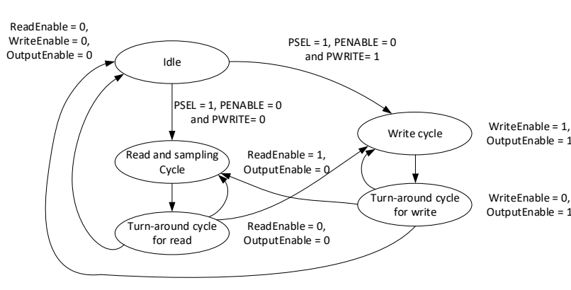
Figure 8.7: State machine to interface APB to asynchronous or tristate buses.
