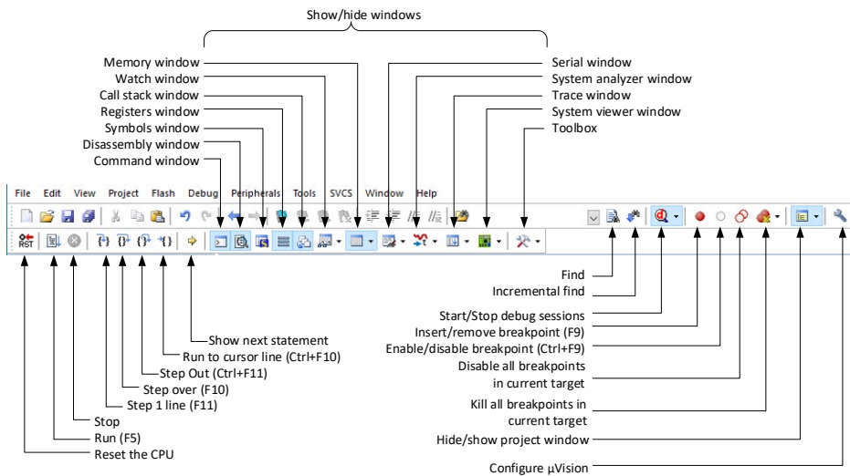
Figure 11.19: Toolbar during debug session.
